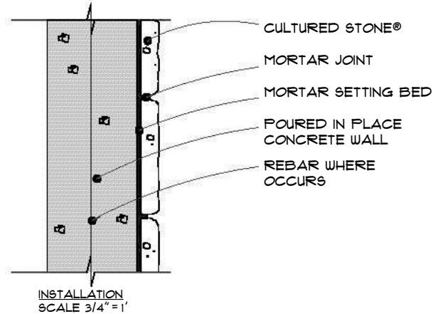
INSTALLATION ON CONCRETE WALL SCALE AS NOTED © 2011 Boral Stone Products LLC
