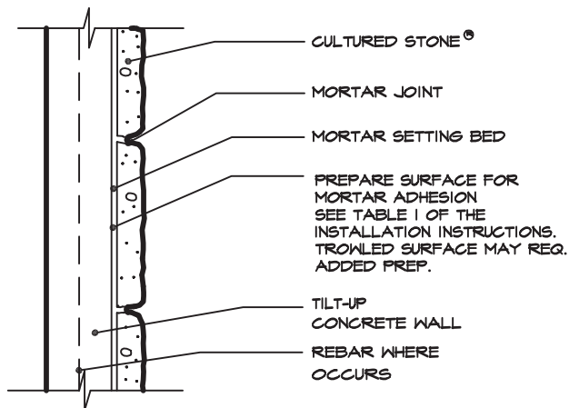
CULTURED STONE® OVER TILT-UP WALL SCALE: 1/2" = 1'-0" © 2011 Boral Stone Products LLC
