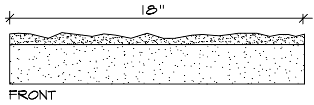
WATERTABLE/SILL PROFILE
